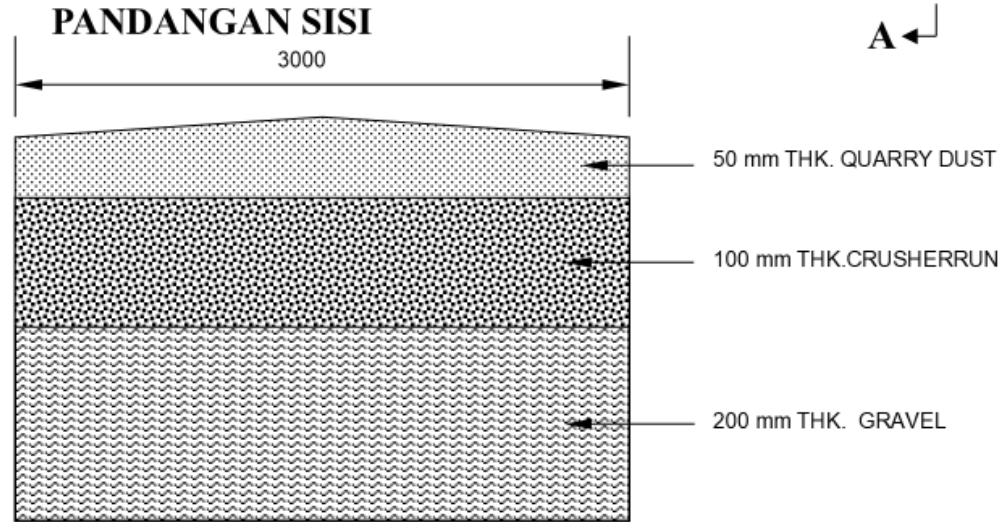
KERATAN A - A
